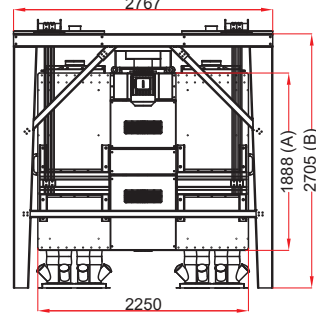
Double Compartment / İki Pasajlı
