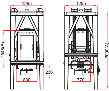
64x64 Single Compartment / Tek Pasajlı
