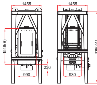
80x80 Single Compartment / Tek Pasajlı
